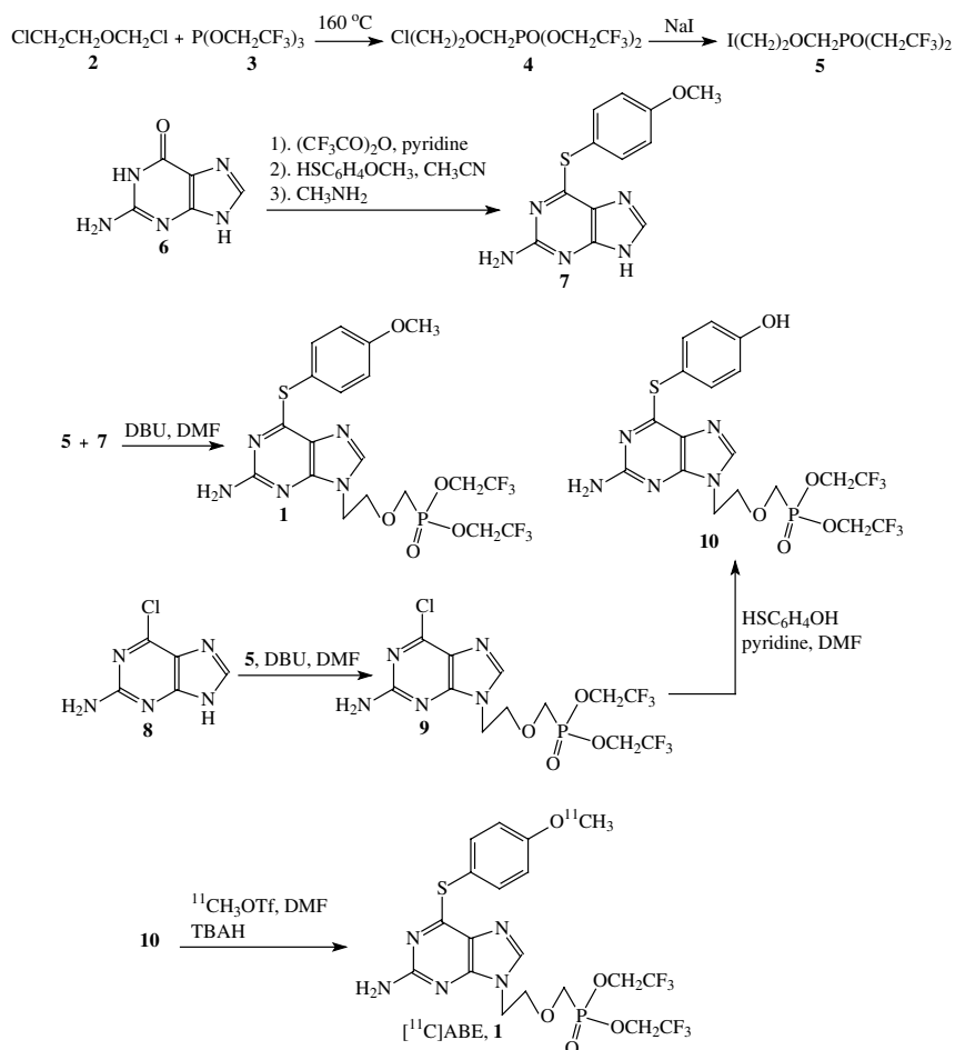
Scheme 1. Synthesis of 2-amino-6-(4-[ ^{11}\text{C} ]methoxyphenylthio)-9-[2-(phosphonomethoxy)ethyl]purine bis(2,2,2-trifluoroethyl) ester ([ ^{11}\text{C} ]ABE, [ ^{11}\text{C} ]1) using unprotected HO-precursor 10.
