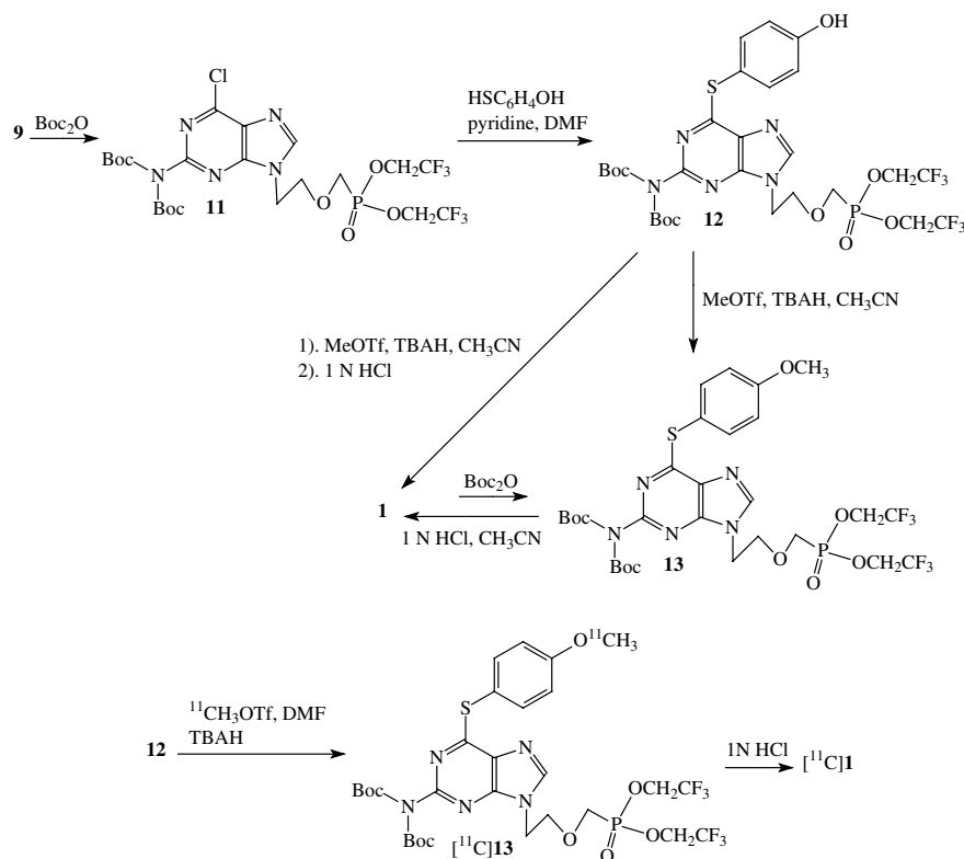
Scheme 2. Synthesis of 2-amino-6-(4-[ ^{11}\text{C} ]methoxyphenylthio)-9-[2-(phosphonomethoxy)ethyl]purine bis(2,2,2-trifluoroethyl) ester ( [^{11}\text{C}]\text{ABE} , [^{11}\text{C}]\mathbf{1} ) using 2- N -Boc protected HO-precursor \mathbf{12} .
